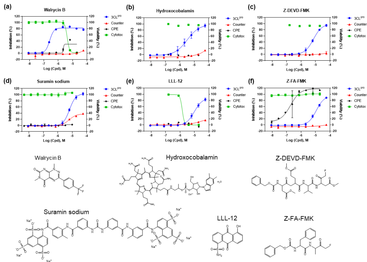
Figure 4. Concentration-response curves of the 6 most potent compounds with IC_{50} values < 15 \mu M and maximal inhibition > 80\% determined in the SARS-CoV-2 3CL pro enzyme assay. Enzyme assay (blue) and counter screen (red) curves correspond to left y-axis showing inhibitory results, CPE (black) and cytotoxicity (green) curves correspond to right y-axis showing cell viability. (a) Walrycin B, IC_{50} = 0.26 \mu M . (b) Hydroxocobalamin, IC_{50} = 3.29 \mu M . (c) Z-DEVD-FMK, IC_{50} = 6.81 \mu M . (d) Suramin sodium, IC_{50} = 6.5 \mu M . (e) LLL-12, IC_{50} = 9.84 \mu M . (f) Z-FA-FMK, IC_{50} = 11.39 \mu M . Primary CPE and cytotoxicity screens were conducted in 4 concentrations, only the hits were further confirmed with 8 concentrations with dilution ratio of 1:3.
